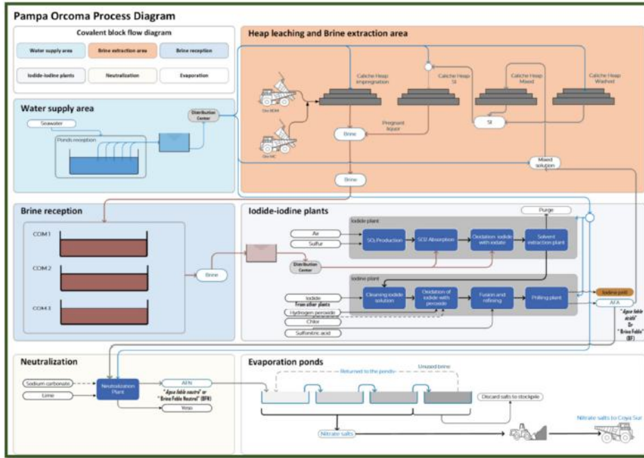
Figure 14-1. Simplified Pampa Orcoma Process Flowsheet
