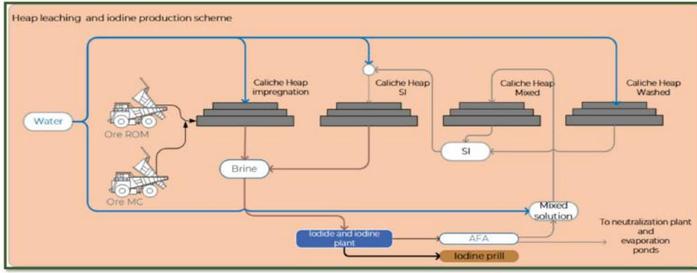
Figure 14-4. Schematic Process Flow of Caliche Leaching
