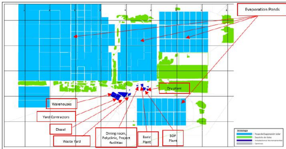
Figure 15-5. Facilities SOP
