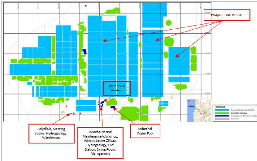
Figure 15-5. Facilities SOP
