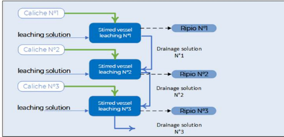
Figure 10-7. Successive Leach Test Development Procedure
