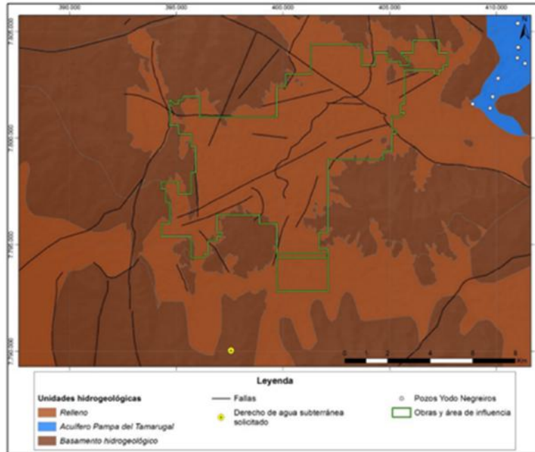
Figure 17-1. Hydrogeological units
